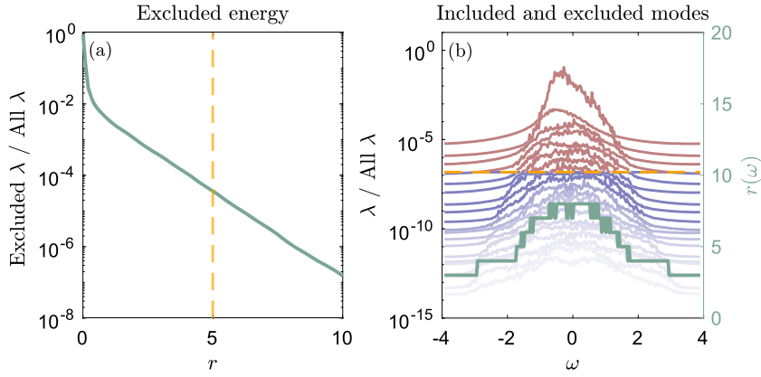
Fig. 4. SPOD energies. (a) The energy not captured by the first rN_\omega modes, calculated as the ratio of the sum of the energies of the excluded modes to the sum of the energies of all the modes. The dashed line corresponds to the r value used to determine the cutoff in (b). (b) The energy of the included (red) and excluded (blue) modes as a function of \omega for r = 5 . Inclusion of a given mode \psi_{km} is determined by whether the associated energy is among the rN_\omega largest energies over all frequencies i.e., whether \lambda_{km} \geq \tilde{\lambda}_{(rN_\omega)} (see (13)). The cutoff energy \tilde{\lambda}_{(rN_\omega)} is shown in orange. The number of modes at each frequency r(\omega) is shown in green on the right axis; the mean is r = 5 . (For interpretation of the references to color in this figure legend, the reader is referred to the web version of this article.)
