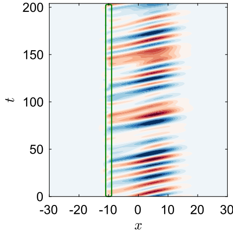
Fig. 3. A trajectory of the (standard) Ginzburg-Landau system with \mu_0 = 0.229 . The green lines demarcate the location of the forcing. The spatiotemporal structure enables space-time modes, like SPOD modes, to represent the trajectory far more efficiently than space-only modes. (For interpretation of the references to color in this figure legend, the reader is referred to the web version of this article.)
