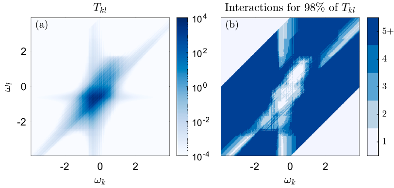
Fig. 11. The impact of \omega_l on \omega_k as defined by (75) via triadic interaction with \omega_i = \omega_k - \omega_l . (a) shows T_{kl} , a proxy for the strength of all interactions between the SPOD modes at \omega_l with those at \omega_i . (b) shows how many of these interactions are needed to account for 98 % of T_{kl} .
