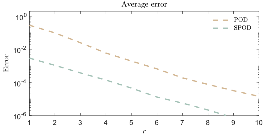
Fig. 1. The relative error for the SPOD and POD trajectory encoders as a function of r , the number of modes used.
