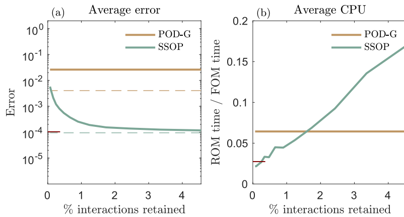
Fig. 13. The relative error (a) and CPU time (b) for the method with r = 5 using the sparse-triadic-interaction approximation of the nonlinearity as a function of the number of triadic interactions retained. The x-axis shows the percentage of the total triadic interactions used. The red ticks indicate results using the DEIM approximation of the nonlinearity. (For interpretation of the references to color in this figure legend, the reader is referred to the web version of this article.)
