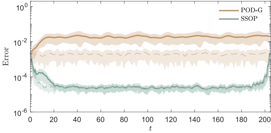
Fig. 5. Error as a function of time for the proposed method and for POD-G, both with r = 5 . The curves represent the mean error over the 30 test trajectories, and the shaded regions indicate the standard deviation of these errors. The dashed curves show the respective projection errors, which serve as lower bounds for the two methods.
