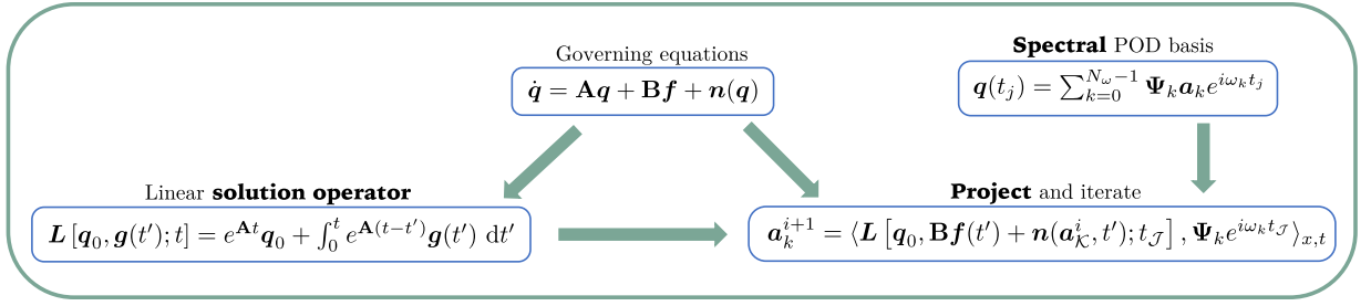
Fig. 2. Spectral solution operator projection: a system of nonlinear algebraic equations is obtained by performing a space-time projection of a linear solution operator onto the set of SPOD modes used to encode trajectories. The linear solution operator returns the solution to the linear system given the initial condition and forcing. Nonlinearities are handled in this framework as a state-dependent forcing. The system is solved via a fixed-point iteration, which may be viewed as a perturbation series around the linear solution.
