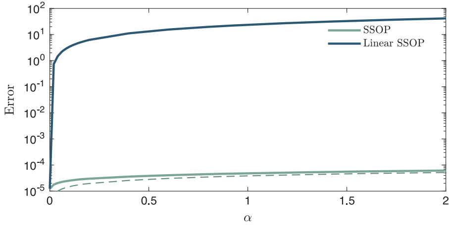
Fig. 10. Error as a function of strength of nonlinear term. As \alpha is increased, the linear SSOP solution deteriorates, but the nonlinear method, which uses the linear solution as an initial guess, retains accuracy.
