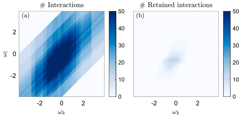
Fig. 12. (a) The total number of interactions between SPOD modes at \omega_l and \omega_k - \omega_l with r = 5 . (b) The number of these interactions that are retained when \epsilon = 10^{-1.8} . Only 1.7% of the interactions in (a) are retained with this threshold.
