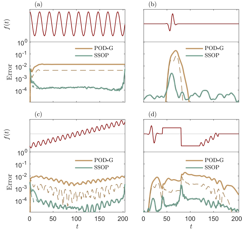
Fig. 8. The error as a function of time for a variety of non-stochastic forcings for both SSOP and POD-G with r = 5 modes, along with the respective projection errors (dashed). The SSOP performance is robust for these out-of-sample forcings.
