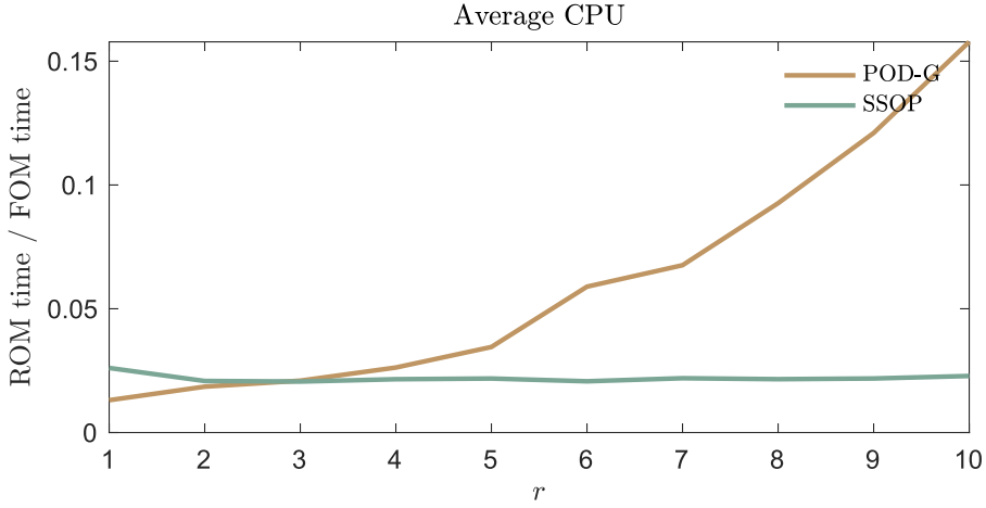
Fig. 7. CPU time for SSOP in comparison to that of POD-G as a function of the number of modes used in the ROMs.
