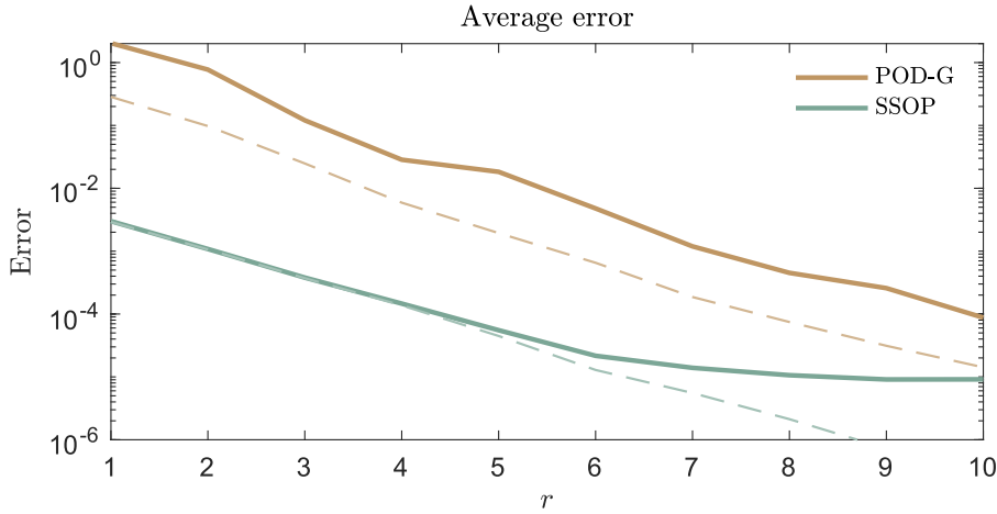
Fig. 6. Error, averaged over time, for SSOP and for POD-G as a function of r , the number of modes used in the ROMs. The dashed curves again represent the projection error onto the POD and SPOD modes.
