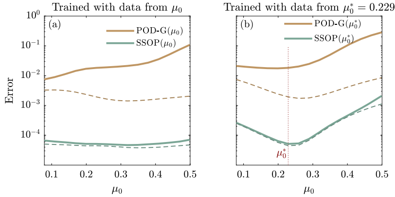
Fig. 9. The methods tested on a range of Ginzburg-Landau systems parameterized by \mu_0 with r = 5 . In (a), the model is trained using data from the same GL system. In (b), the models are trained using data from \mu_0^* = 0.229 . The dashed curves correspond to the projection error for the modes from the training system.
