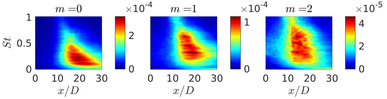
Figure 5. RMS of LES pressure fluctuations of the M_j = 1.5 jet at radial surface r/D = 6 from St = [0, 1] and x/D = [0, 30] for three azimuthal wavenumbers, m = [0, 2] .
