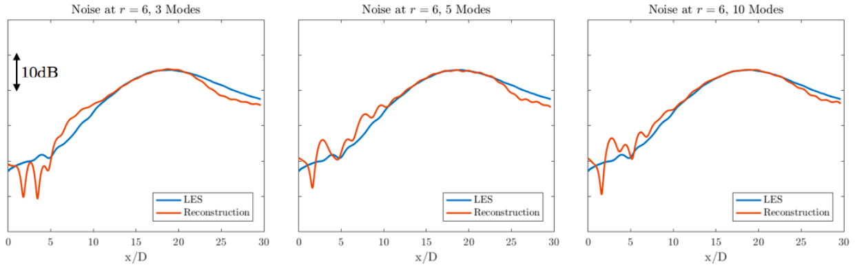
Figure 4. Comparison of pressure RMS values by dB at r/D = 6 for the LES ensemble and reconstructions in the resolvent basis using 3, 5, and 10 resolvent modes.
