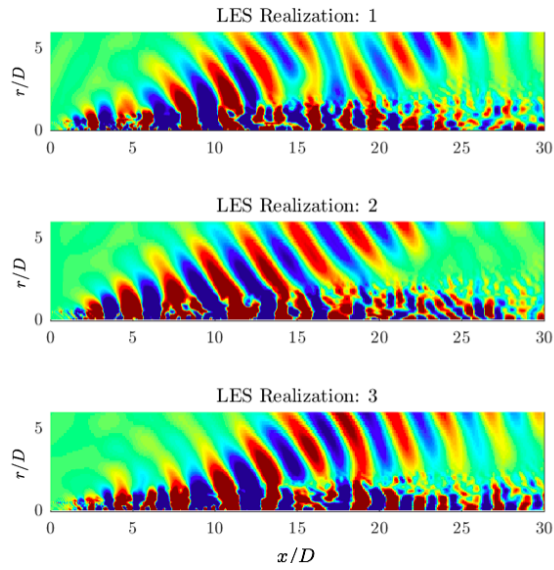
Figure 2. Three realizations of the LES pressure field at M_j = 1.5 , St = 0.26 , m = 0 . Red and blue contours vary from \pm 50\% of the maximum fluctuating pressure of each mode, \pm 0.5 \|q_{p'}\|_\infty .
