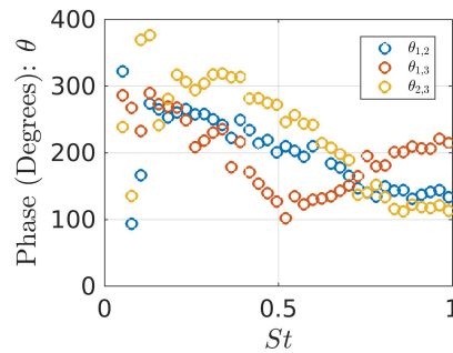
Figure 18. Phases of the three covariance matrix angles as a function of frequency.
