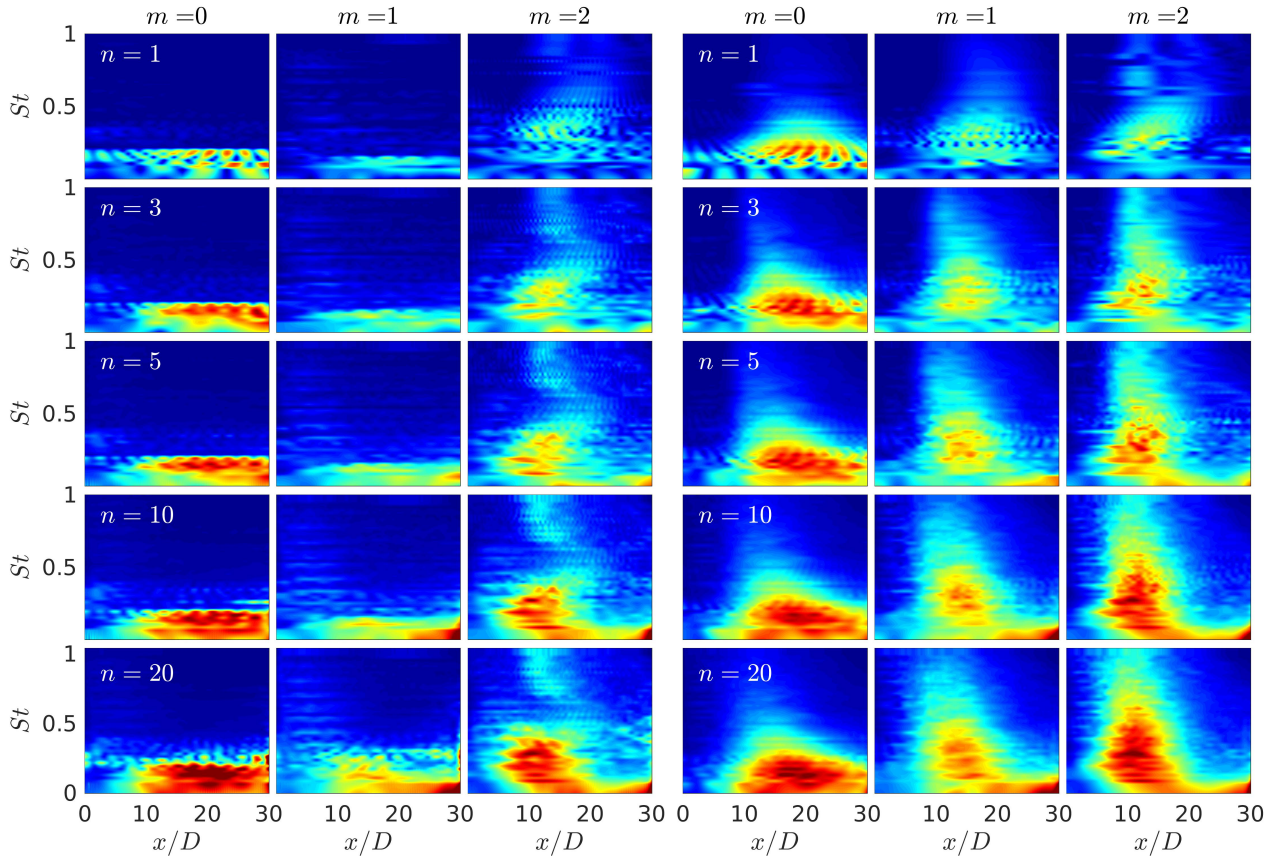
Figure 8. RMS of resolvent reconstructions of the M_j = 0.9 jet, without an eddy-viscosity model (left) and with a RANS eddy-viscosity model (right), at radial surface r/D = 6 from St = [0, 1] and x/D = [0, 30] for three azimuthal wavenumbers, m = [0, 2] , from left to right and using n = 1, 3, 5, 10, 20 modes from top to bottom. Contours and axes mirror those of figure 7.
