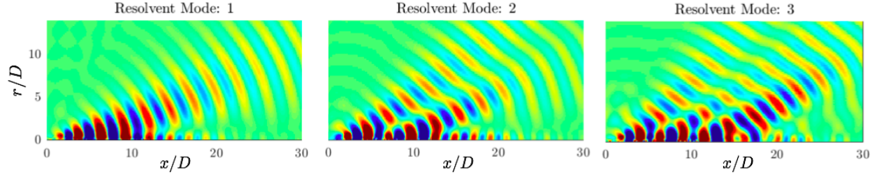
Figure 1. The first three resolvent modes of fluctuating pressure, q_p' . Red and blue contours vary from \pm 50\% of the maximum fluctuating pressure of each mode, \pm 0.5\|q_p'\|_\infty . M_j = 1.5 , St = 0.26 , m = 0 .
