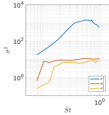
Figure 16. Resolvent gains for the first three modes across St = [0, 1] for azimuthal wavenumber m = 0 .
