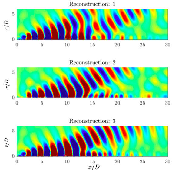
Figure 3. Reconstructions of the corresponding LES realizations using the 3-mode resolvent basis. Contour values are identical to figure 2. M_j = 1.5 , St = 0.26 , m = 0 .
