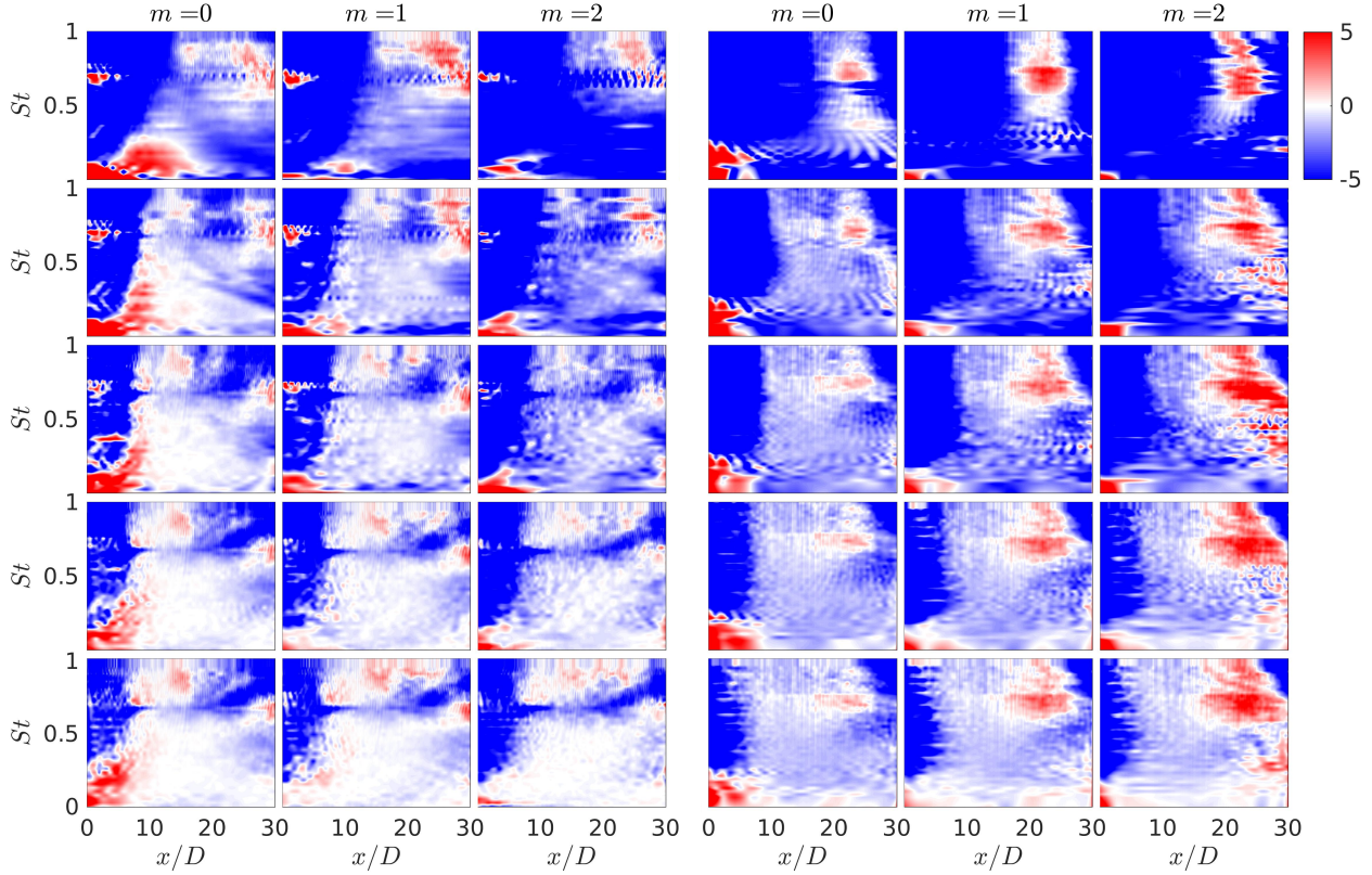
Figure 9. Difference in decibels, dB , between the RMS values of LES and the eddy-viscosity resolvent reconstructions for the M_j = 1.5 jet. Axes mirror those of figure 5 with contours set at \pm 5 dB.
