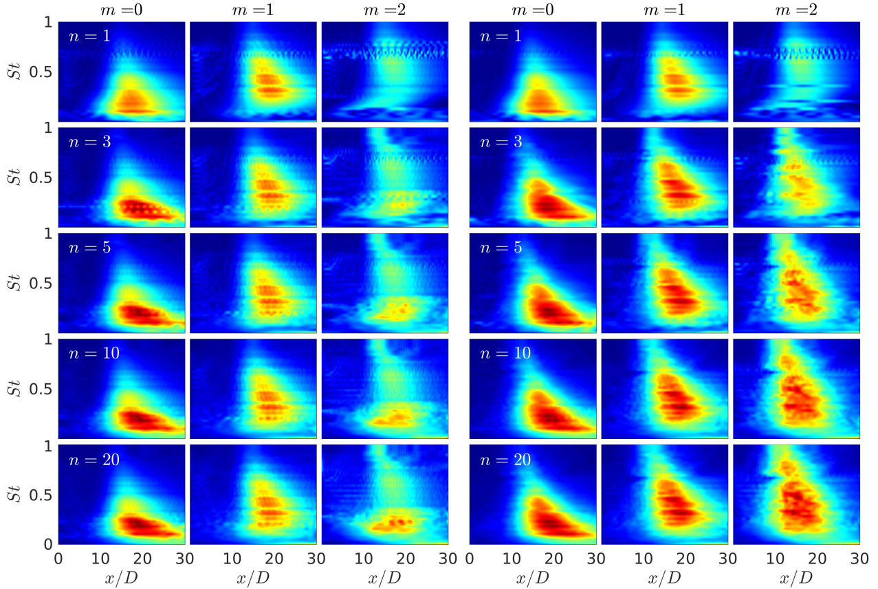
Figure 6. RMS of resolvent reconstructions of the M_j = 1.5 jet, without an eddy-viscosity model (left) and with a RANS eddy-viscosity model (right), at radial surface r/D = 6 from St = [0, 1] and x/D = [0, 30] for three azimuthal wavenumbers, m = [0, 2] , from left to right and using n = 1, 3, 5, 10, 20 modes from top to bottom. Contours and axes mirror those of figure 5.
