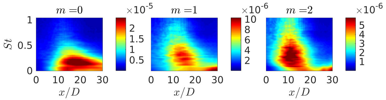
Figure 7. RMS of LES pressure fluctuations of the M_j = 0.9 jet at radial surface r/D = 6 from St = [0, 1] and x/D = [0, 30] for three azimuthal wavenumbers, m = [0, 2] .
