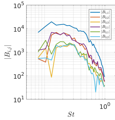
Figure 14. Magnitudes of the six unique entries of the 3 \times 3 covariance matrix for azimuthal wavenumber, m = 0 .
