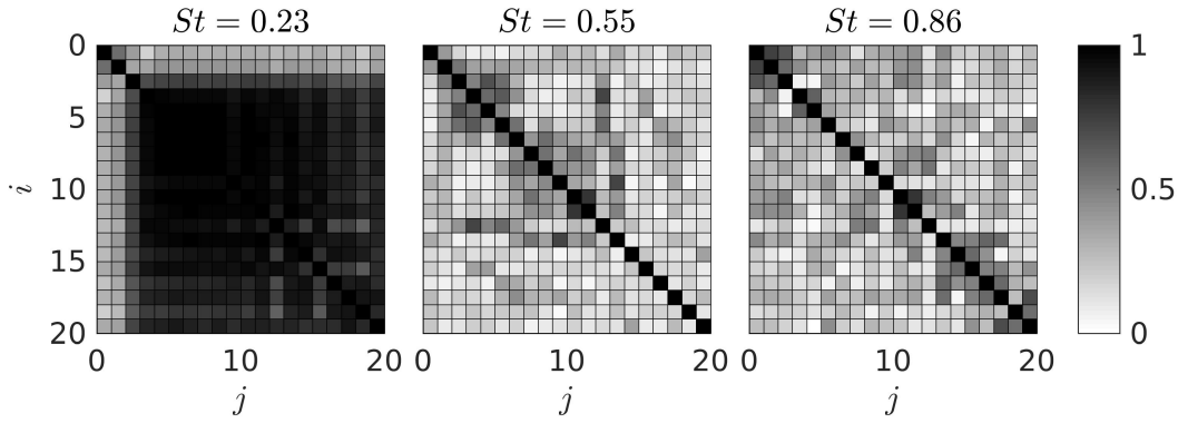
Figure 13. Normalized magnitude of the estimated forcing CSD, \tilde{\mathbf{B}}_{norm} = \text{diag}(\tilde{\mathbf{B}})^{-1/2} \tilde{\mathbf{B}} \text{diag}(\tilde{\mathbf{B}})^{-1/2} .
