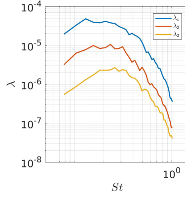
Figure 15. Three largest eigenvalues of the SPOD spectrum computed over the LES acoustic domain, C_z for azimuthal wavenumber m = 0 .
