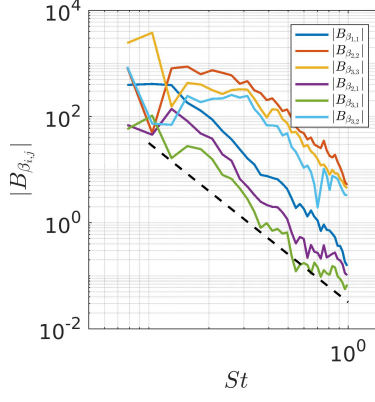
Figure 17. Magnitude of the forcing projection coefficients, \beta_k/\beta_k^* = \tilde{V}^* W_f f_k f_k^* W_f \tilde{V} . The dashed line gives \sim St^{-3} .
